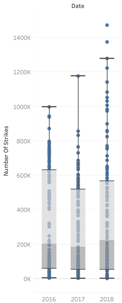
Boxplot
